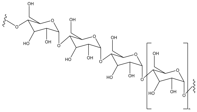
Polysaccharide
