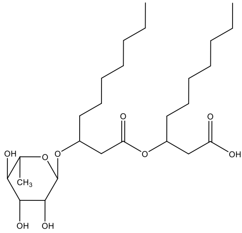
Glycolipids
