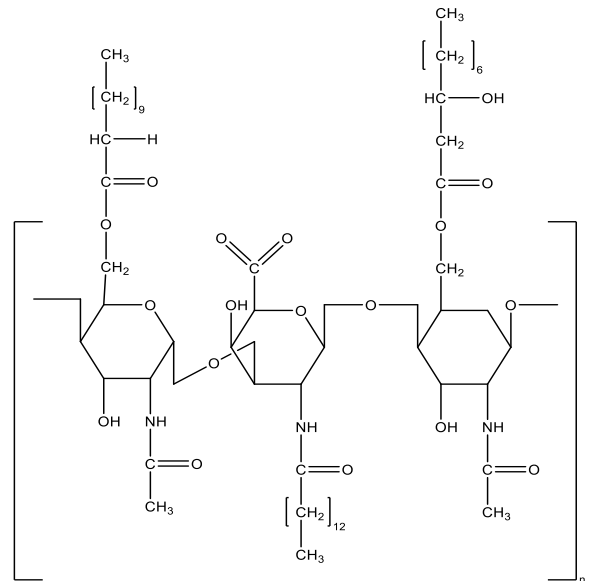
Polymeric
