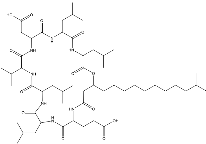
Lipopeptides
